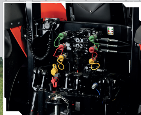
Up to 3 spool valves with flow regulator.
